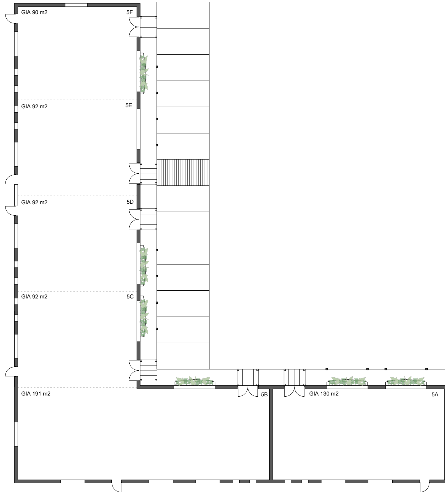
PROPOSED FLOOR PLAN SCALE 1:200 @ a3
